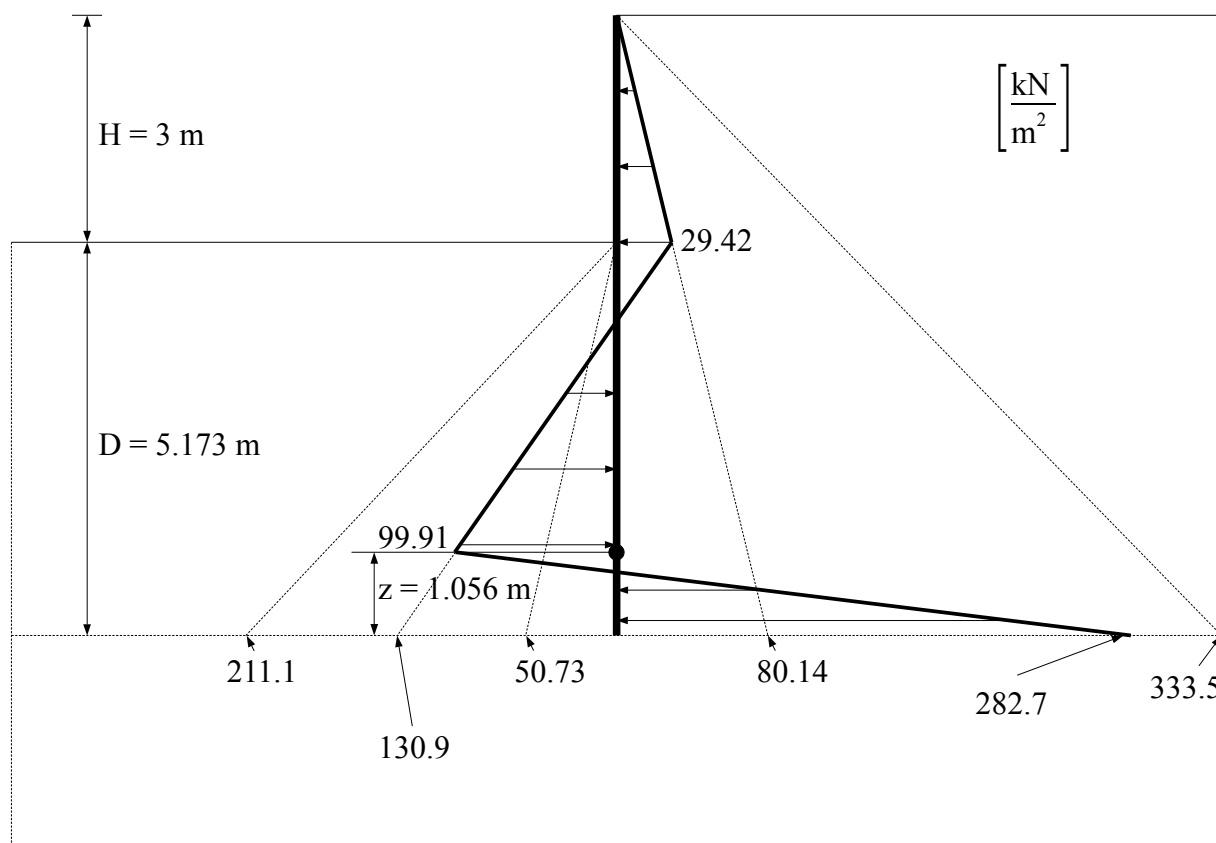
Figure 5.70 – The quantitative values of depth [m] and resultant earth pressures [ \text{kN/m}^2 ] on the wall
