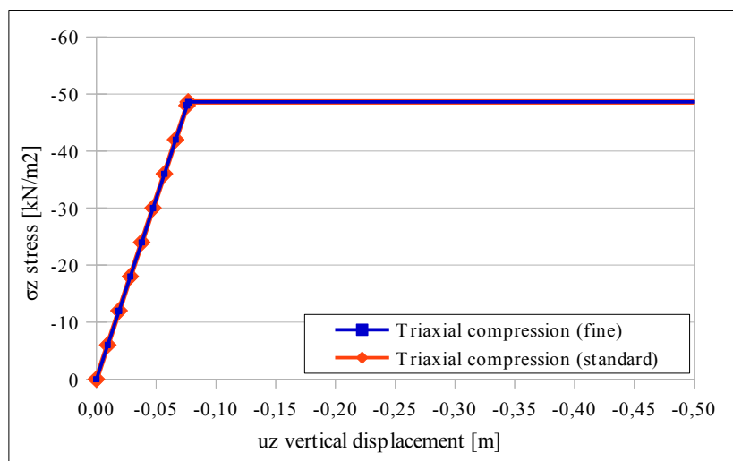
Figure 5.35 – Stress-displacement diagram
